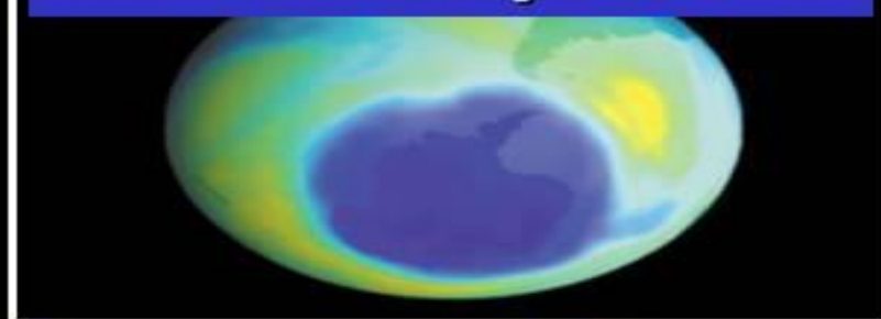
Ozone Depletion
